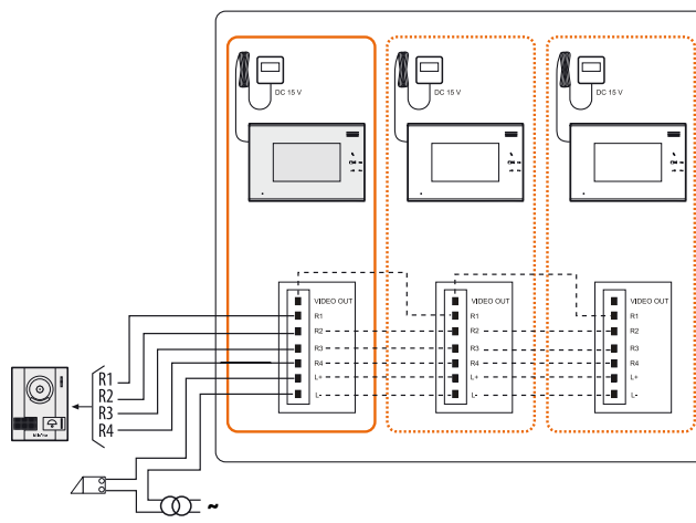
WIRING DIAGRAM (THE DOTTED LINES REPRESENT THE DIAGRAM FOR ADDITIONAL VIDEO HANDSETS)
