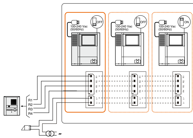
WIRING DIAGRAM (THE DOTTED LINES REPRESENT THE DIAGRAM FOR ADDITIONAL VIDEO HANDSETS)
